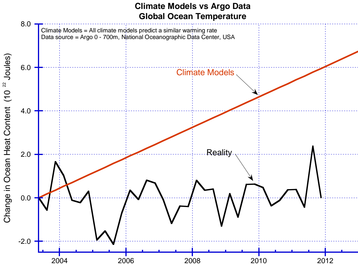
Figure 5: Climate model predictions 14 of ocean temperature, versus the measurements by Argo 15 . The unit of the vertical axis is 10 22 Joules (about 0.01°C).
